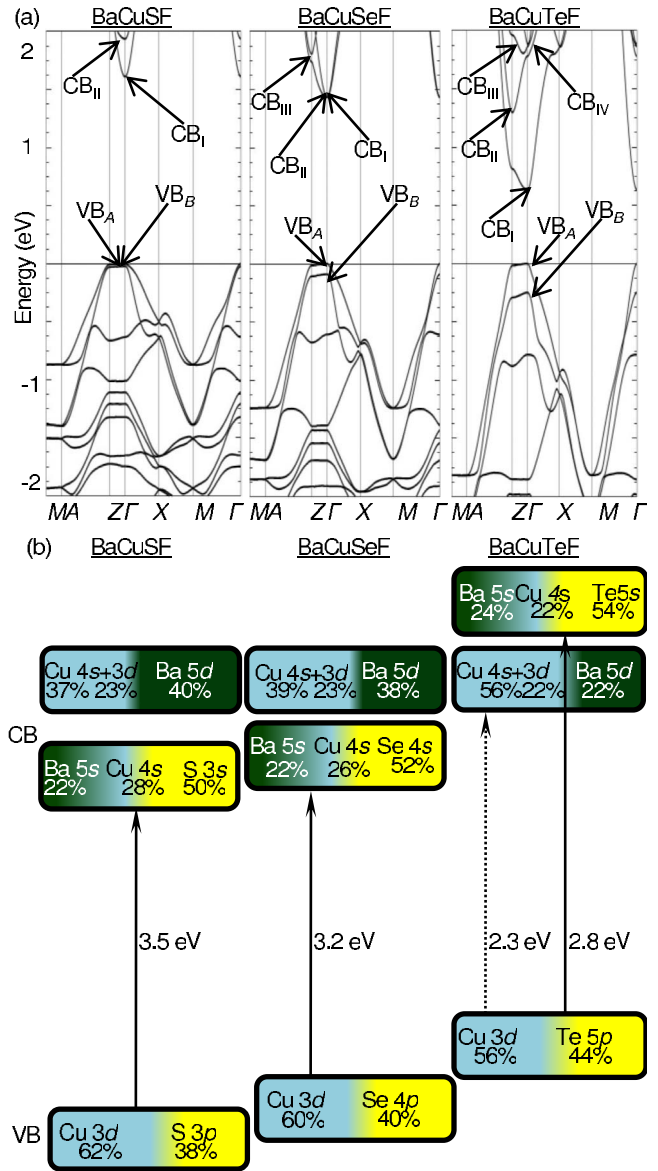
FIG. 1. (Color online) (a) Relativistic band structure of BaCuChF calculated by GGA DFT. The spin-orbit split valence bands are labeled VB_A and VB_B , while the conduction bands are labeled CB_I , CB_{II} , CB_{III} , and CB_{IV} . (b) Schematic electronic structure of BaCuChF compounds. The band gaps in (b) are calculated using the GW approximation.
