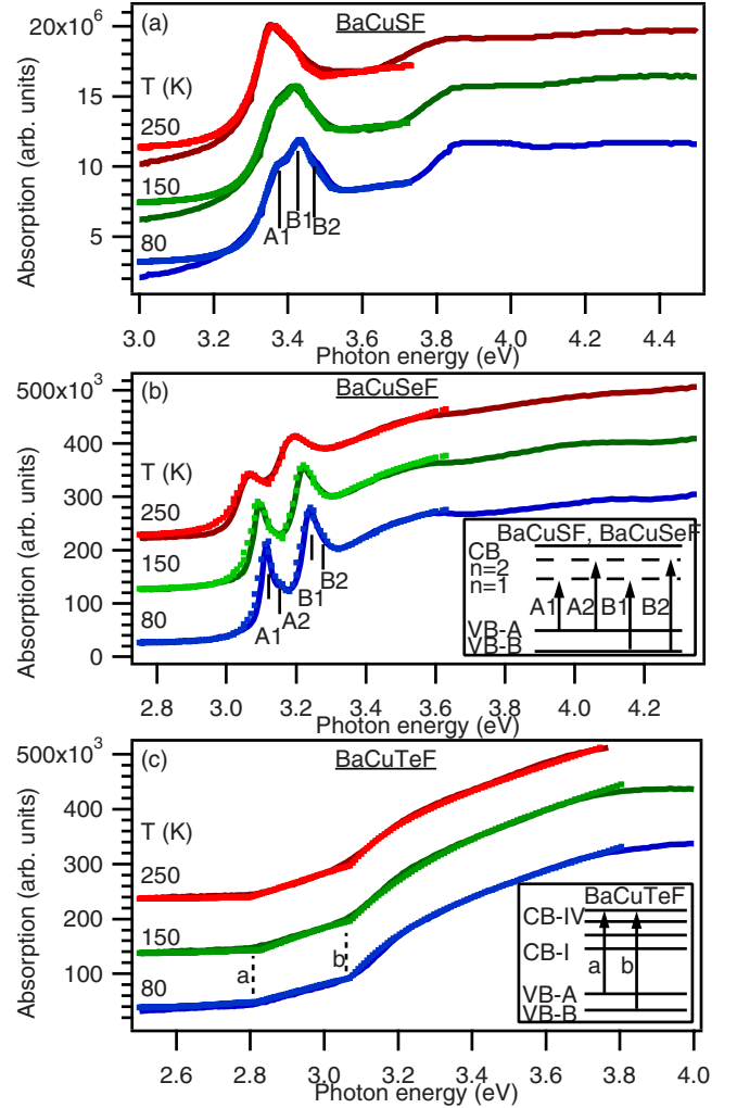
FIG. 3. (Color online) Experimental absorption spectra of (a) \text{BaCuSF} , (b) \text{BaCuSeF} and (c) \text{BaCuTeF} at 80–250 K. The dotted lines are fits based on the analysis described in the text. The spectra are offset on the vertical axis for clarity. Insets: schematic interpretation of the absorption spectra.
